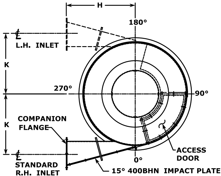
VIEW E-E
